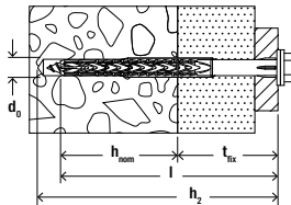
Frame fixing SXRL-FUS
