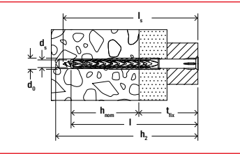
Frame fixing SXRL
