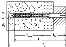
Frame fixing SXRL-T
