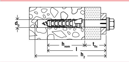
Frame fixing SXR-FUS
