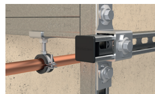
Supported frame construction: PFUF, PFCN, HK, FCN Clix P PFUF, PFCN, HK, FCN Clix P
