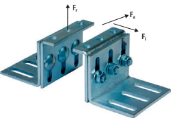
FFPK Saddle max. recom. loads radial F_r = 42000 N lateral F_l = 17500 N
