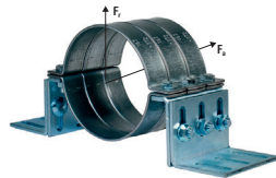
Fixpoint 3 clamps Max. recom. load axial F_a = 16500 N radial F_r = 13980 N
