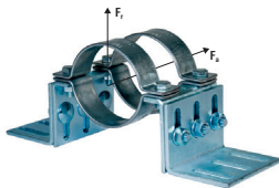
Fixpoint 2 clamps Max. recom. load axial F_a = 11000 N radial F_r = 9320 N
