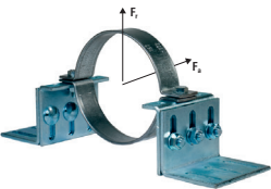
Fixpoint 1 clamp Max. recom. load axial F_a = 5500 N radial F_r = 4660 N
