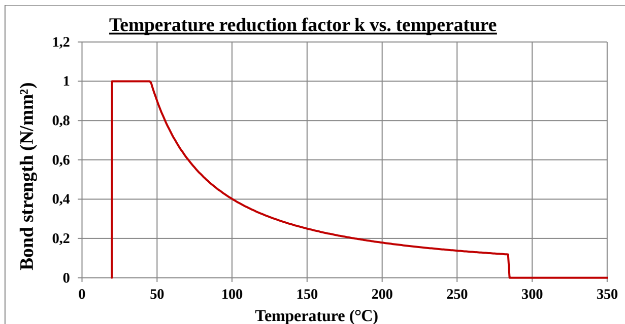
Figure 3 : Temperature reduction factor k(\theta) vs. temperature
